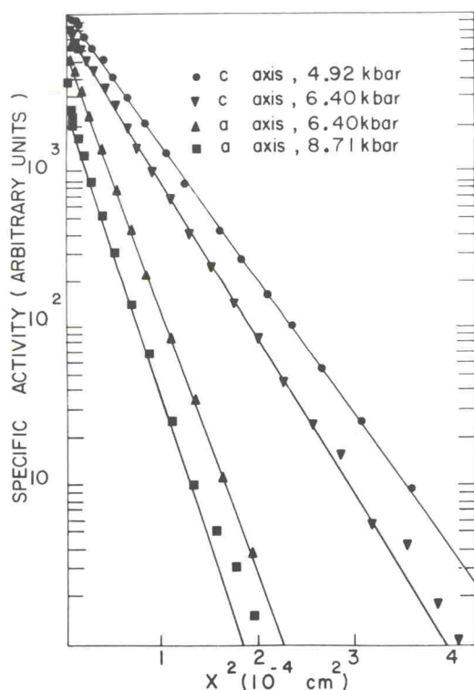
FIG. 1. Best and worst penetration profiles for self-diffusion in zinc at 350.7 °C.
